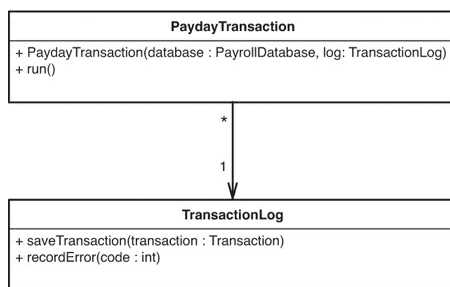
Figure 25.5 PaydayTransaction depending on TransactionLog .
