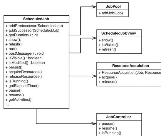
Figure 20.12 ScheduledJob with extracted classes.
