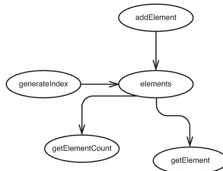
Figure 11.8 Effect sketch of the InMemoryDirectory class.
