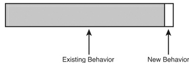
Figure 1.1 Preserving behavior.
