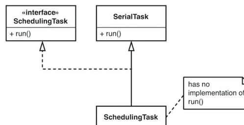
Figure 9.3 SchedulingTask .
