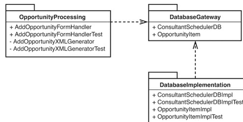
Figure 7.5 Package structure.
