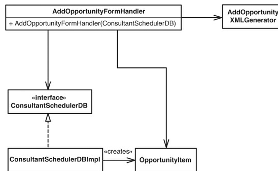
Figure 7.2 Extracting an implementer on ConsultantSchedulerDB .
