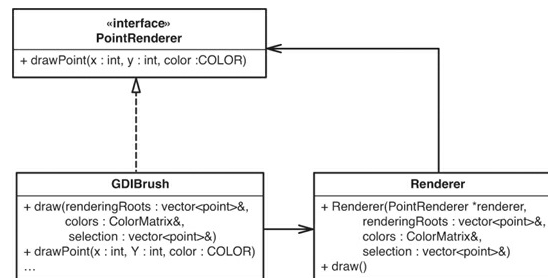
Figure 25.1 GDIBrush after Break Out Method Object.
