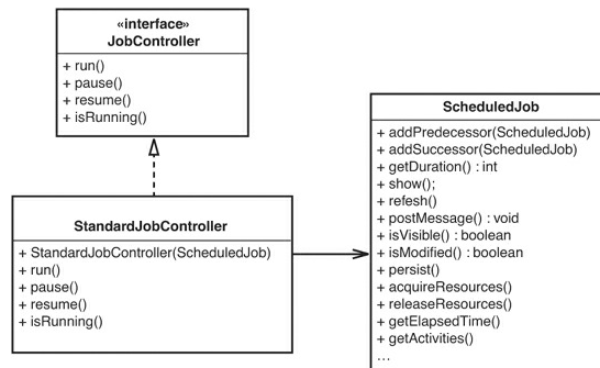
Figure 20.14 Segregating the interface of ScheduledJob .
