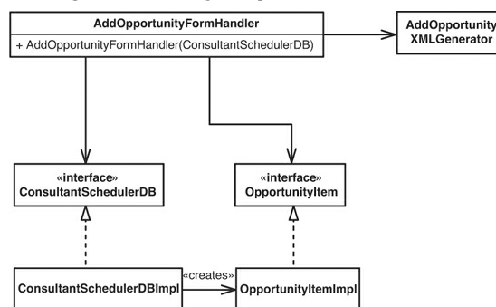
Figure 7.3 Extracting an implementer on OpportunityItem .
