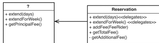
Figure 20.8 Reservation using a new class.
