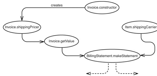
Figure 12.5 Billing system effect sketch.
