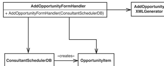
Figure 7.1 Opportunity handling classes.
