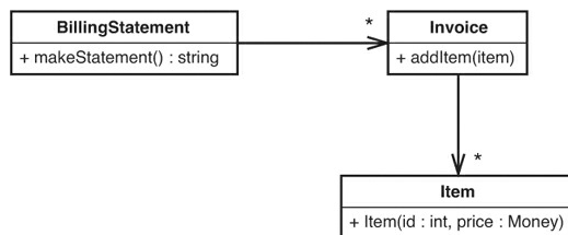
Figure 12.4 Expanded billing system.
