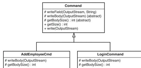
Figure 21.4 Pulling up getSize .
