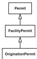
Figure 9.4 The Permit hierarchy
