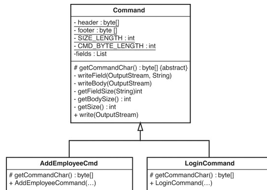
Figure 21.5 Command hierarchy with duplication pulled up.
