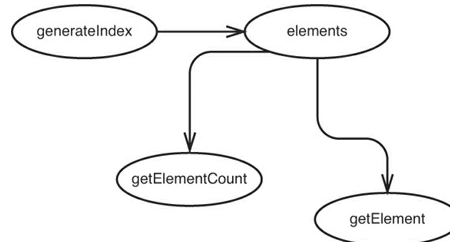
Figure 11.6 Further effects of changes in generateIndex .
