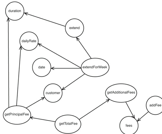
Figure 20.7 A cluster in Reservation .
