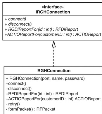
Figure 9.2 RGHConnection after extracting an interface
