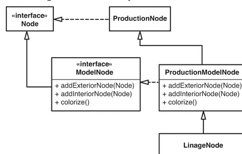
Figure 25.4 Extract Implementer on ModelNode .
