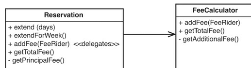
Figure 20.10 Reservation using FeeCalculator .
