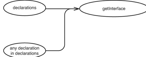
Figure 11.3 Things that affect getInterface .
