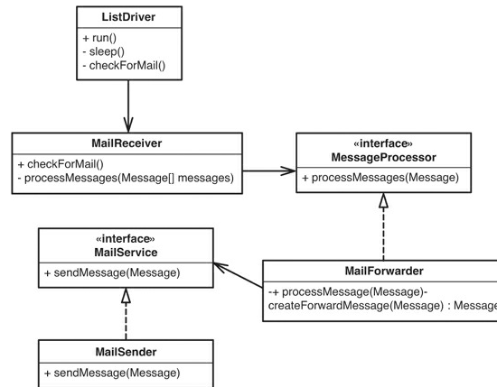
Figure 15.1 A better mailing list server.
