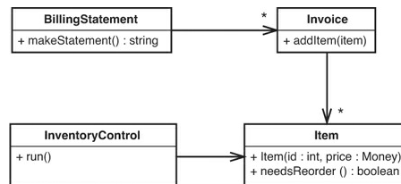
Figure 12.6 Billing system with inventory.
