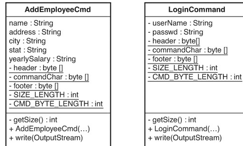
Figure 21.1 AddEmployeeCmd and LoginCommand.
