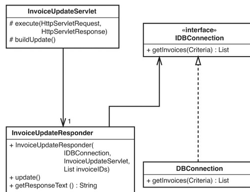
Figure 2.2 Invoice update classes with dependencies broken.
