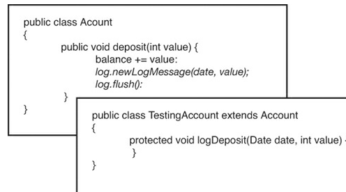
Figure 25.6 TestingAccount superimposed on Account.
