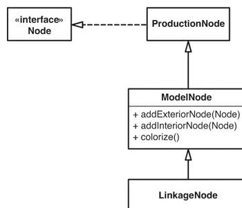
Figure 25.3 After Extract Implementer on Node .
