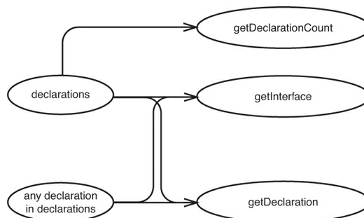
Figure 11.12 Effect sketch for CppClass .
