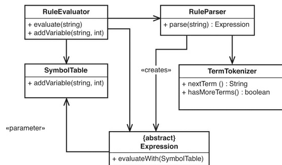
Figure 20.2 Rule classes with responsibilities separated.
