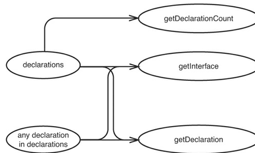
Figure 11.11 Effect sketch for CppClass .
