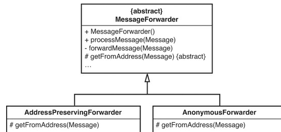
Figure 8.7 Normalized hierarchy.
