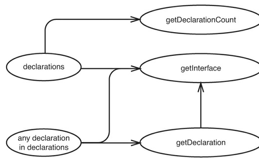
Figure 11.13 Effect sketch for Changed CppClass .
