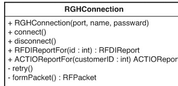
Figure 9.1 RGHConnection .
