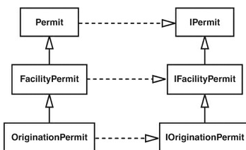
Figure 9.5 Permit hierarchy with extract interfaces.
