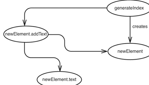
Figure 11.9 Effects through the Element class.
