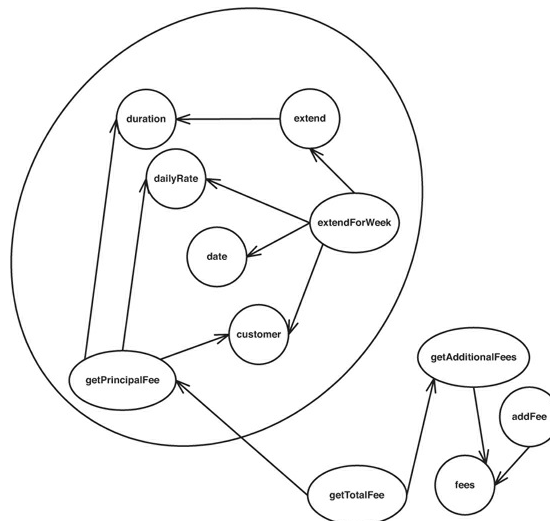
Figure 20.7 A cluster in Reservation .
