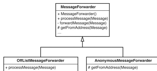
Figure 8.2 Subclassing for two differences.
