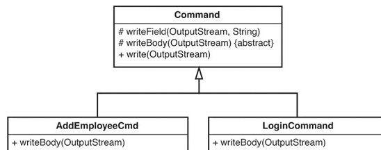
Figure 21.3 Pulling up writeField.
