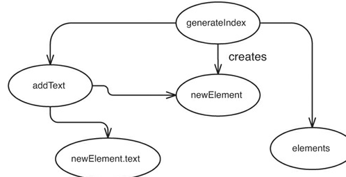
Figure 11.10 generateIndex affecting the elements collection.
