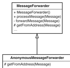
Figure 8.1 Subclassing MessageForwarder .
