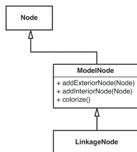
Figure 25.2 ModelNode with superclass and subclass.
