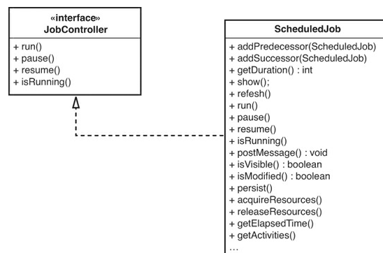
Figure 20.13 A client-specific interface for ScheduledJob .
