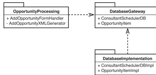
Figure 7.4 Refactored package structure.
